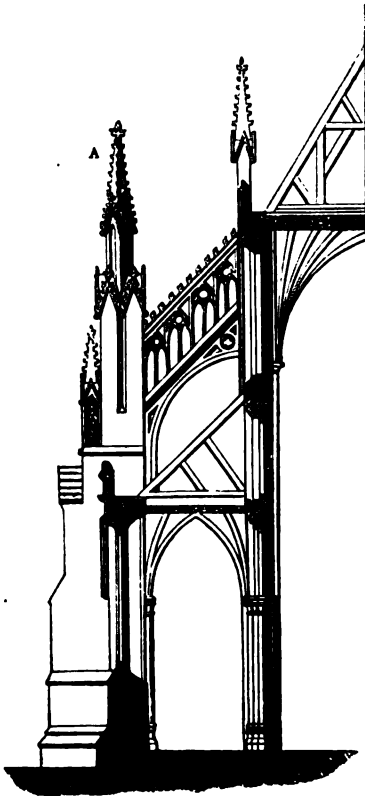
Section of a Pointed Church, with the Flying Buttresses decorated.
