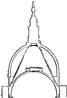
Section of the Dome of St. Paul's.
